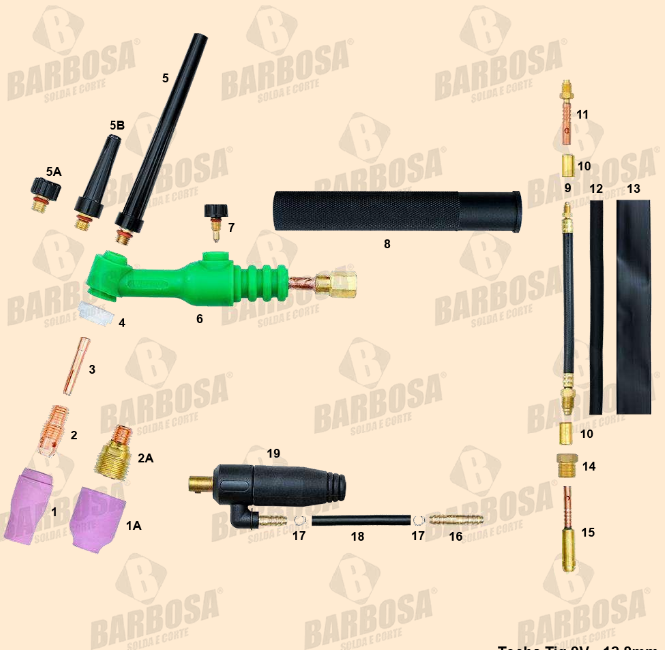
Tocha Tig 9V - 12.8mm
